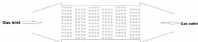
Figure 14. The considered two-dimensional mode for the type B exchanger for drawing in the GAMBIT software
